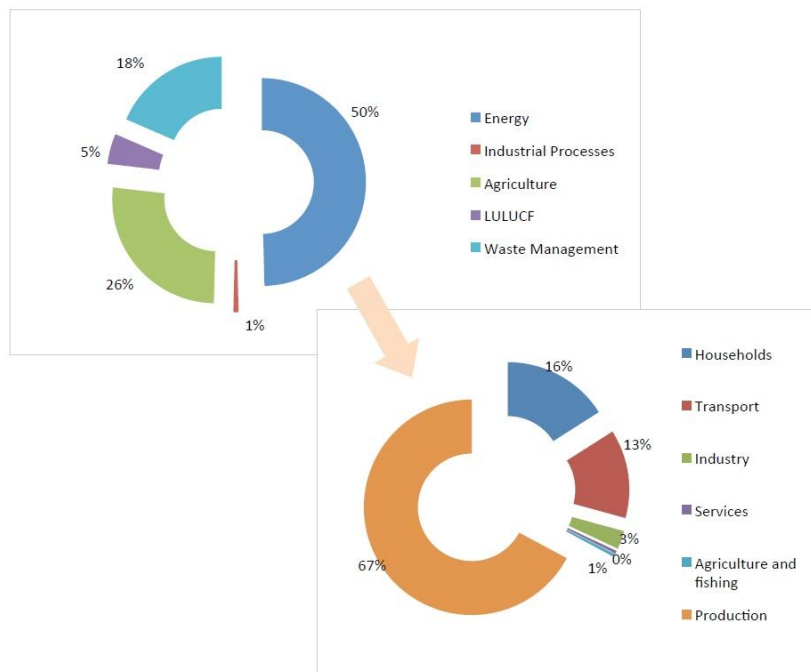
Figure 7: Distribution of the Mitigation Effort in Each Ector over the Period 2020-2030, to Achieve the Conditional Emissions Reduction Objective
