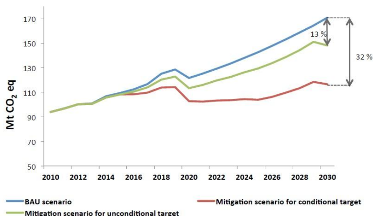
Figure 6: BAU and Mitigation Scenarios
