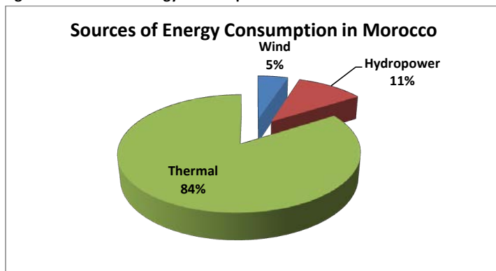
Figure5: Sources of Energy Consumption in Morocco
