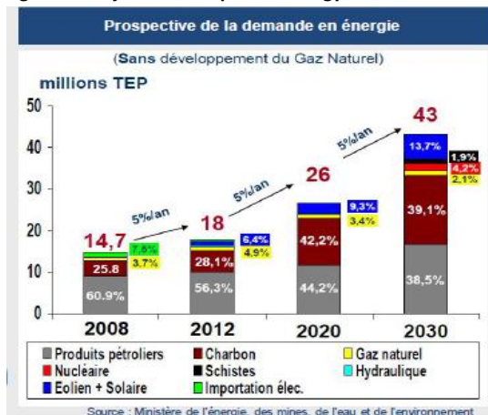
Figure 4: Projection of Expected Energy Demand in Morocco by 2030
