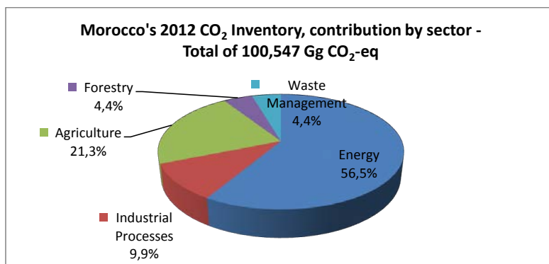
Figure 2: Morocco's total CO 2 Emissions for 2012 and Contribution by Sector
